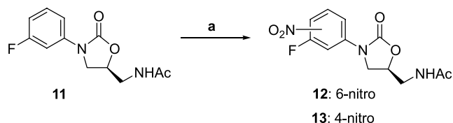
Scheme 4. Nitration of 11 . Reagents and conditions: (a) \text{KNO}_3 , \text{H}_2\text{SO}_4 , 0\text{ }^\circ\text{C} to rt, 4 h.
