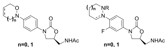
Figure 2. Pseudo-isomers of linezolid and eperzolid.
