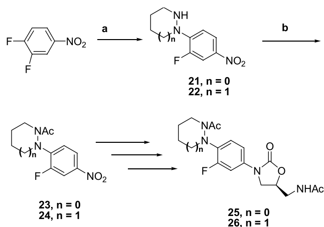
Scheme 7. Synthesis of 25 and 26 . Reagents and conditions: (a) i Pr 2 NEt, and pyrazolidine or hexahydro-pyridazine, CH 3 CN, 90 °C, 10 h; (b) Ac 2 O, pyridine, DMAP, THF, rt, 1 h.
