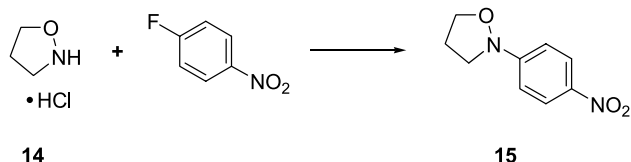
Scheme 5. Isoxazolidine analog.
