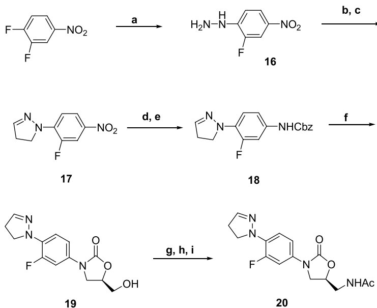
Scheme 6. Synthesis of 2-pyrazoline analog 20 . Reagents and conditions: (a) hydrazine hydrate, pyridine, rt, 50 min; (b) NaH, 1,3-dibromopropane, DMF, 0\text{ }^\circ\text{C} to rt, 3 h; (c) air; (d) 10% \text{Pd}/\text{C} , \text{HCO}_2\text{NH}_4 , THF/MeOH (1:2); (e) CbzCl, \text{NaHCO}_3 , \text{H}_2\text{O}/\text{acetone} (1:2), 0\text{ }^\circ\text{C} to rt, 2 h; (f) n -BuLi, ( R )-glycidyl butyrate, THF, -78\text{ }^\circ\text{C} to rt, 18 h; (g) MsCl, \text{NEt}_3 , \text{CH}_2\text{Cl}_2 , rt, 1 h; (h) \text{NH}_4\text{OH} , THF, i PrOH, 100\text{ }^\circ\text{C} , 5 h, sealed tube; (i) \text{Ac}_2\text{O} , triethylamine, \text{CH}_2\text{Cl}_2 , rt, 2 h.
